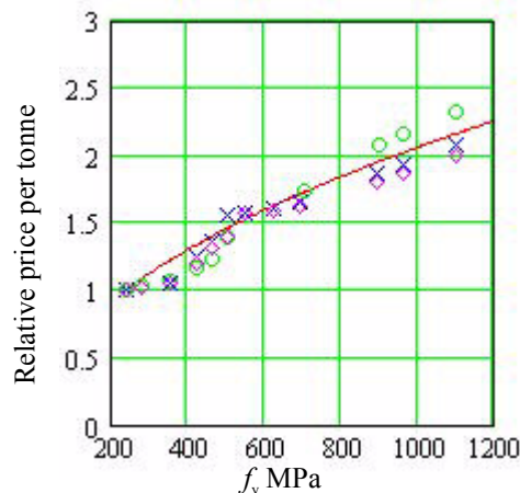
Fig. 1. Approximate price per tonne of hot rolled steel normalised with price of S235 as function of yield strength.
