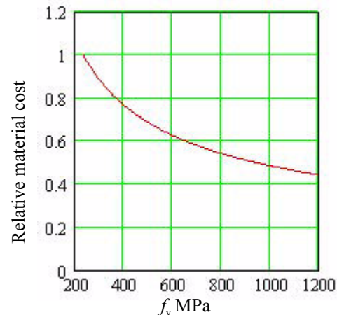
Fig. 2. Approximate material cost normalised with the cost of S235 assuming that the strength can be fully utilised.
