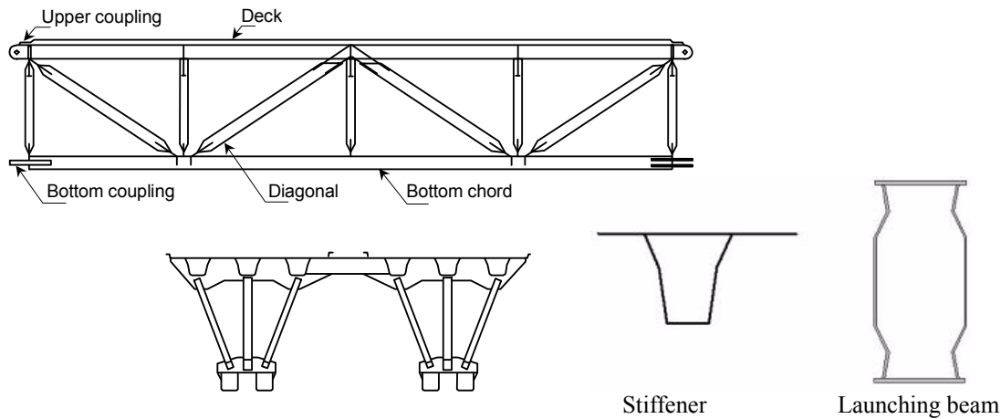
Fig. 11. Truss element for Fast Bridge 48 developed by Karlskronavarvet AB, Sweden.
