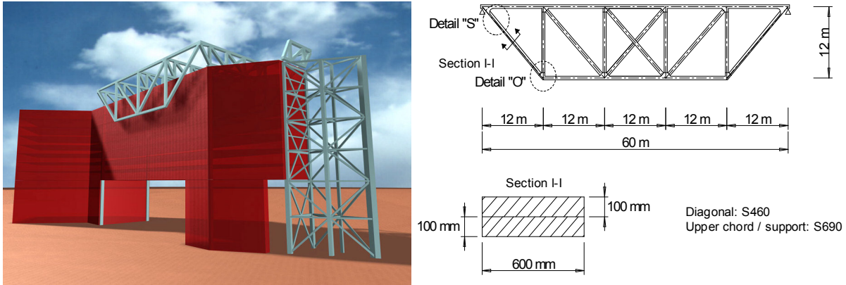
Fig. 9. Truss structure in the Sony Center.
