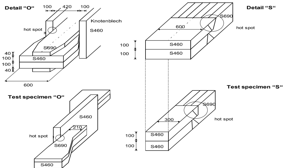
Fig.10. Structural detailing and large scale specimens.
