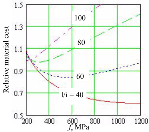
Fig. 3. Relative material cost for column subject to flexural buckling (curve a) as function of yield strength f_y . Reference cost is for steel S235.
