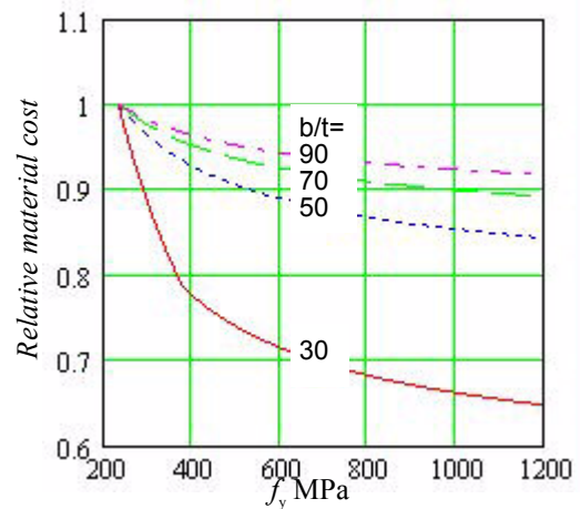
Fig. 4. Relative cost for a plate supported along all edges and subject to uniform compression as function of yield strength f_y . Reference cost is for steel S235.
