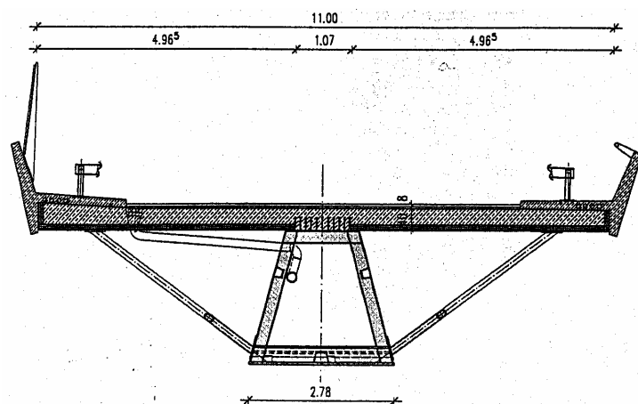
Fig. 8. Cross section of the Nesenbachtalbrücke.
